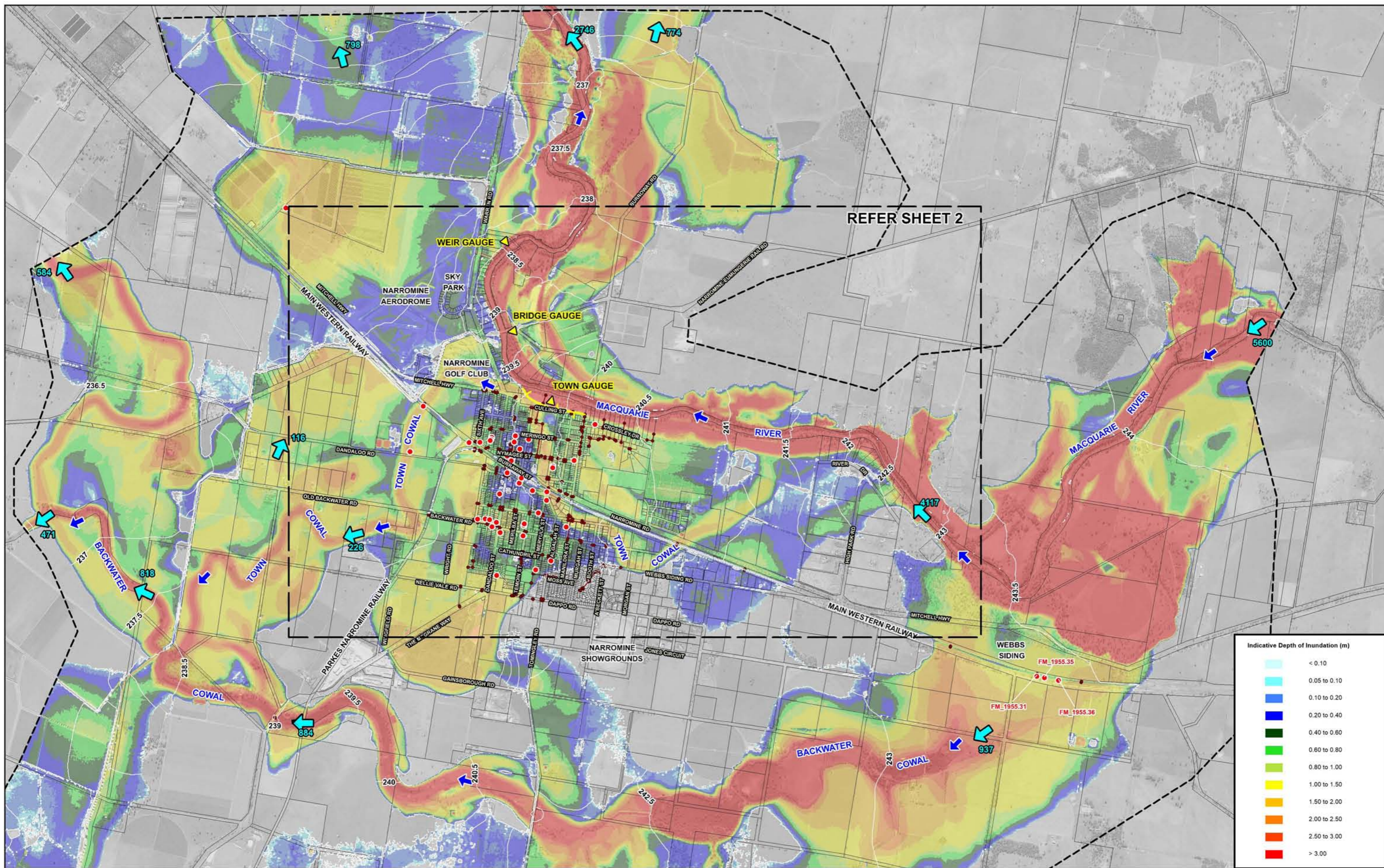
NARROMINE TOWN FLOODPLAIN RISK MANAGEMENT STUDY AND PLAN UPDATE Figure 2.4 (Sheet 1 of 2) INDICATIVE EXTENT AND DEPTH OF MAIN STREAM FLOODING FEBRUARY 1955 FLOOD
