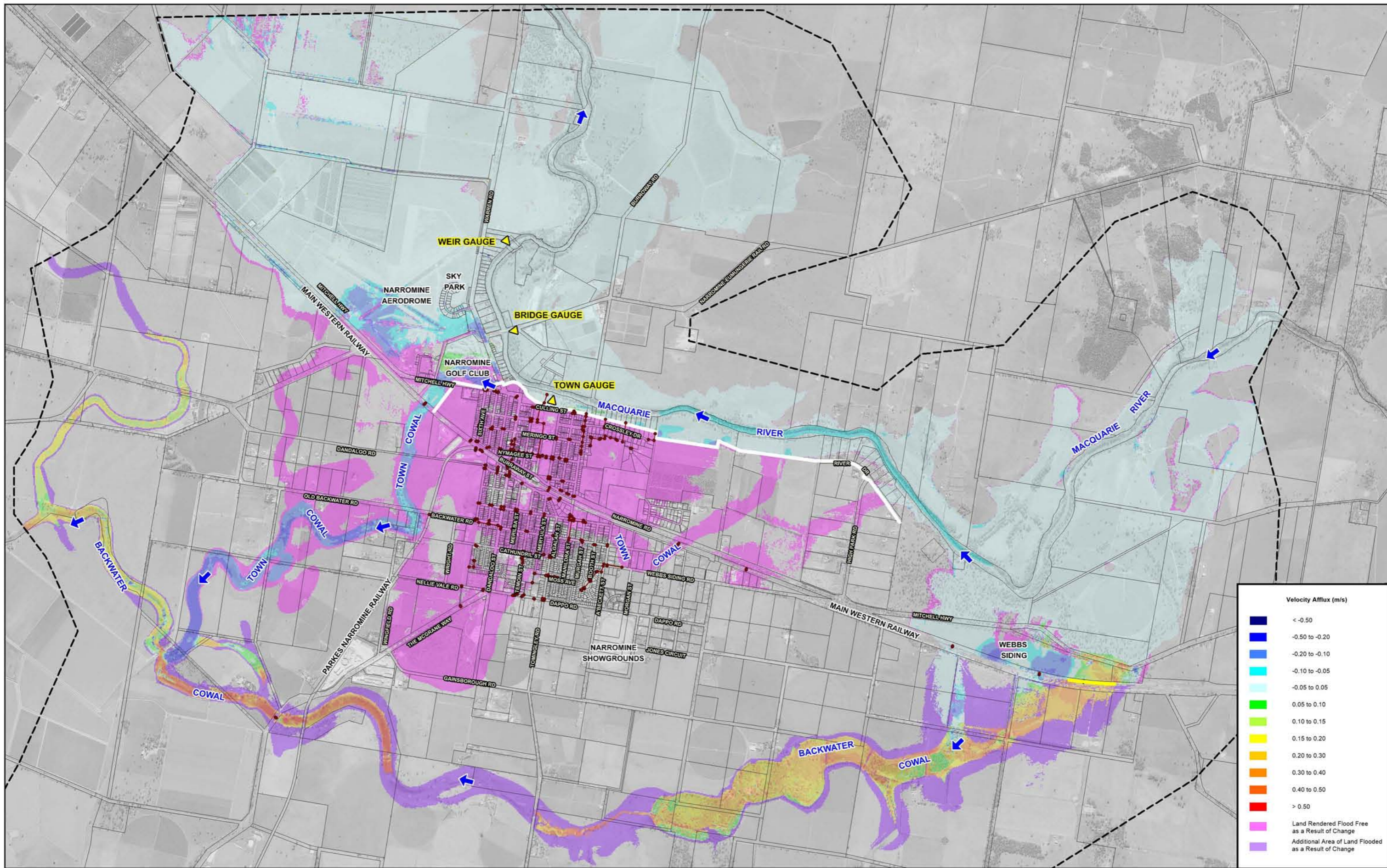
NARROMINE TOWN FLOODPLAIN RISK MANAGEMENT STUDY AND PLAN UPDATE Figure C1.16 IMPACT OF LEVEE OPTION B1A WITH RAILWAY CULVERT UPGRADE ON MAXIMUM MAIN STREAM FLOODING FLOW VELOCITIES 1% AEP
