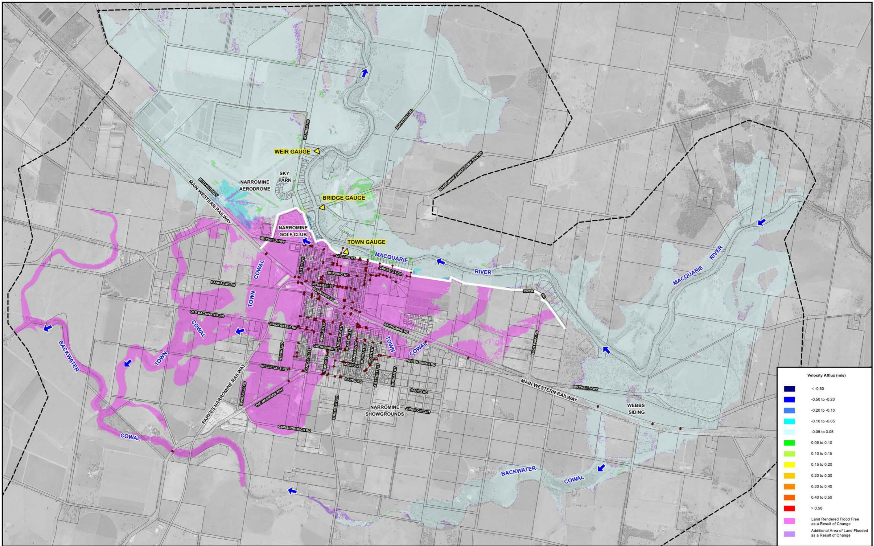
NARROMINE TOWN FLOODPLAIN RISK MANAGEMENT STUDY AND PLAN UPDATE Figure C1.8 IMPACT OF LEVEE OPTION B2 ON MAXIMUM MAIN STREAM FLOODING FLOW VELOCITIES 1% AEP
