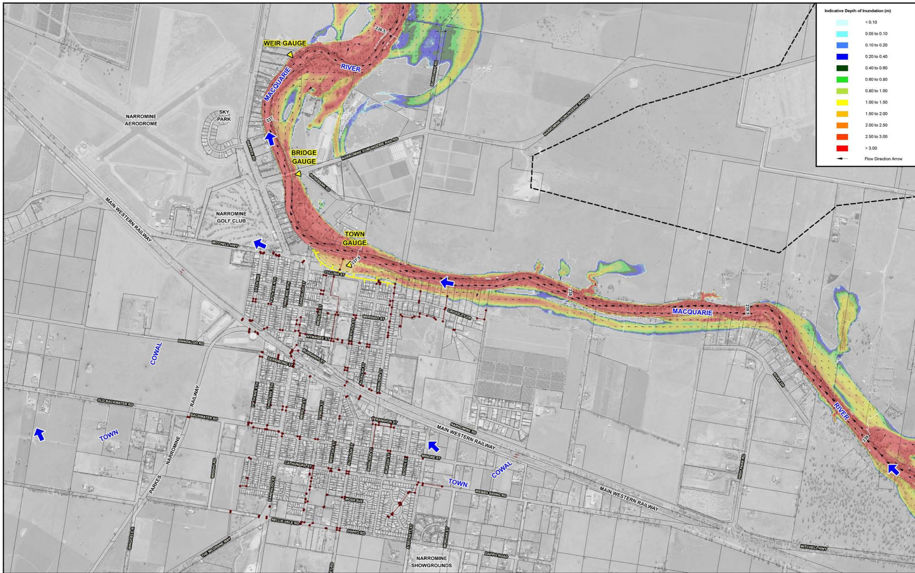
Figure 2.9 (Sheet 2 of 2) INDICATIVE EXTENT AND DEPTH OF MAIN STREAM FLOODING 5% AEP
